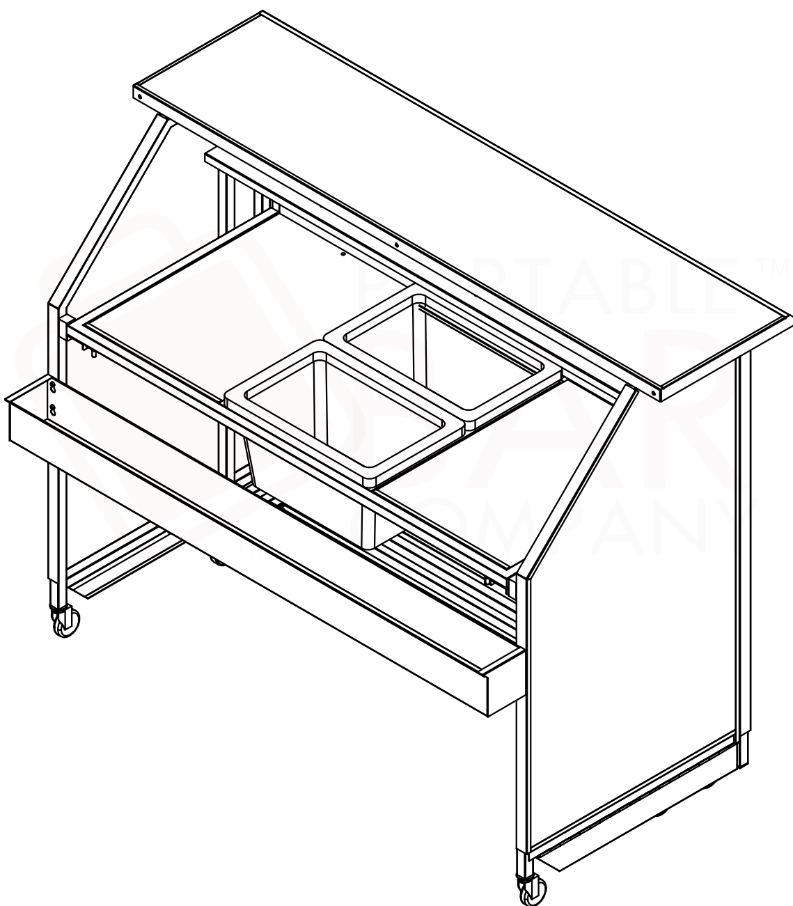
Figure 10. Full Assembly.
