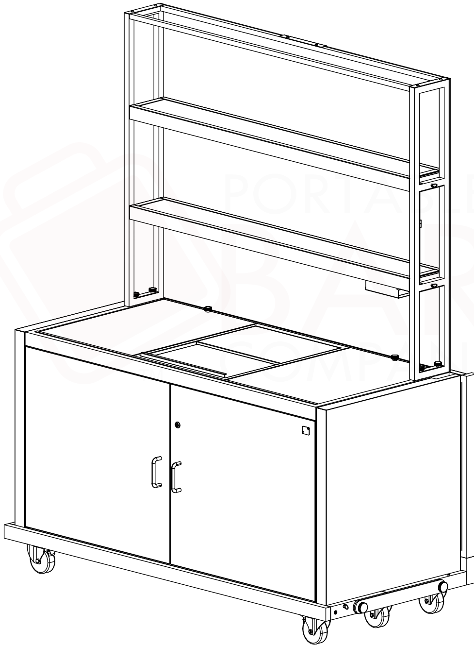
Figure 4. Full Assembly
